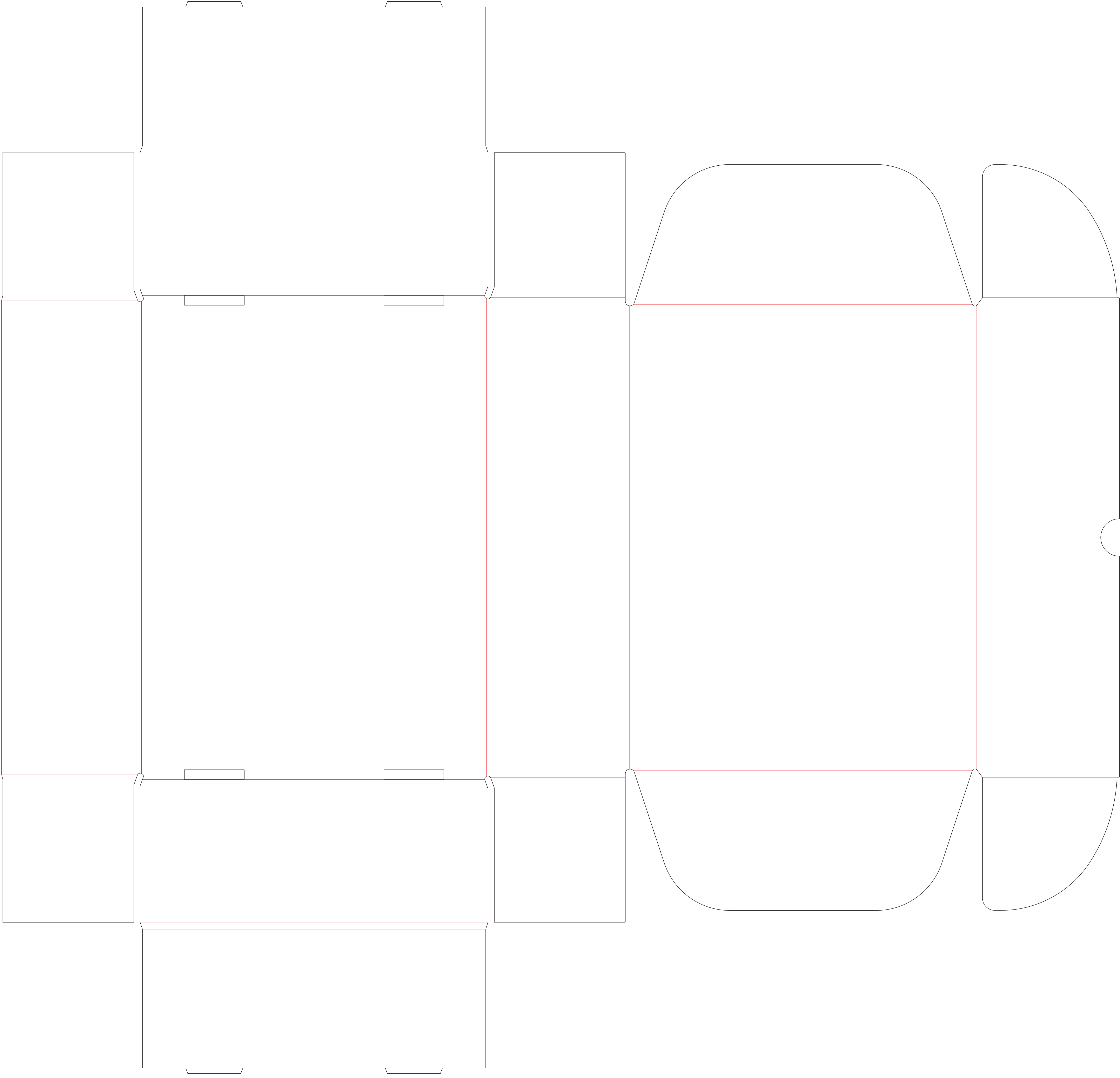
Box 300x220x90 mm OUTSIDE
